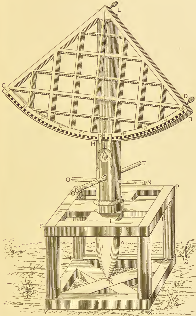
FIG. 18.—Early out-door quadrant of Tycho; for observing altitudes by help of the sights D , L and the plumb line.
